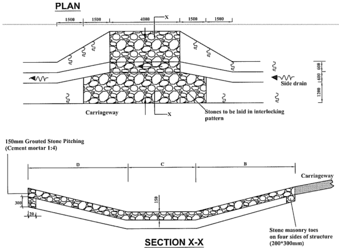
FIGURE C18-ACCESS DRIFT
