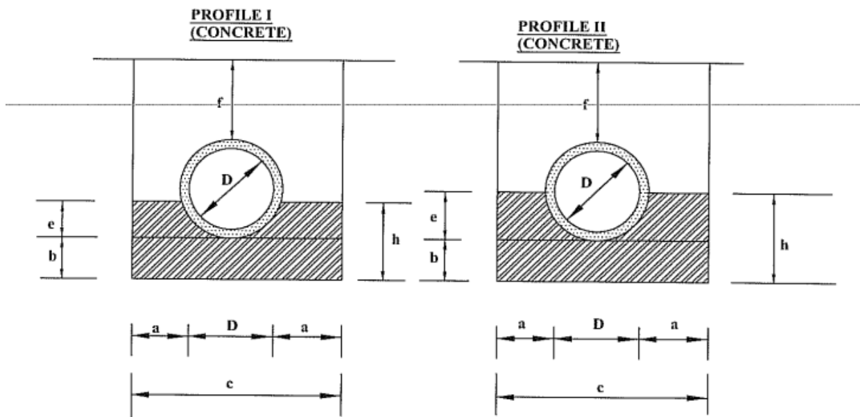
FIGURE C16-BEDDING AND HAUNCH PROFILE TYPES I &amp; II
