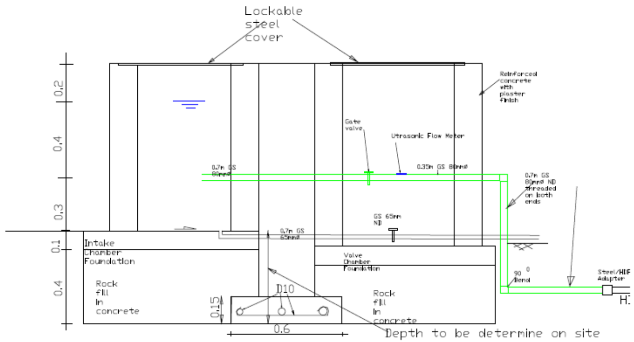
Intake & Valve Chamber Section SCALE : 1:100
